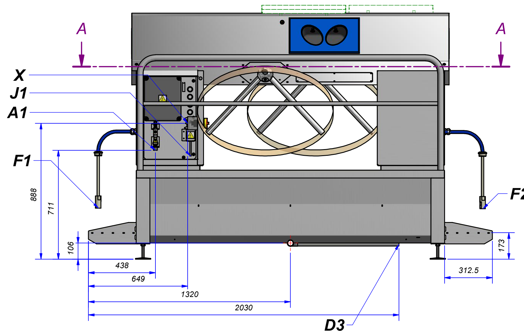
Front view
