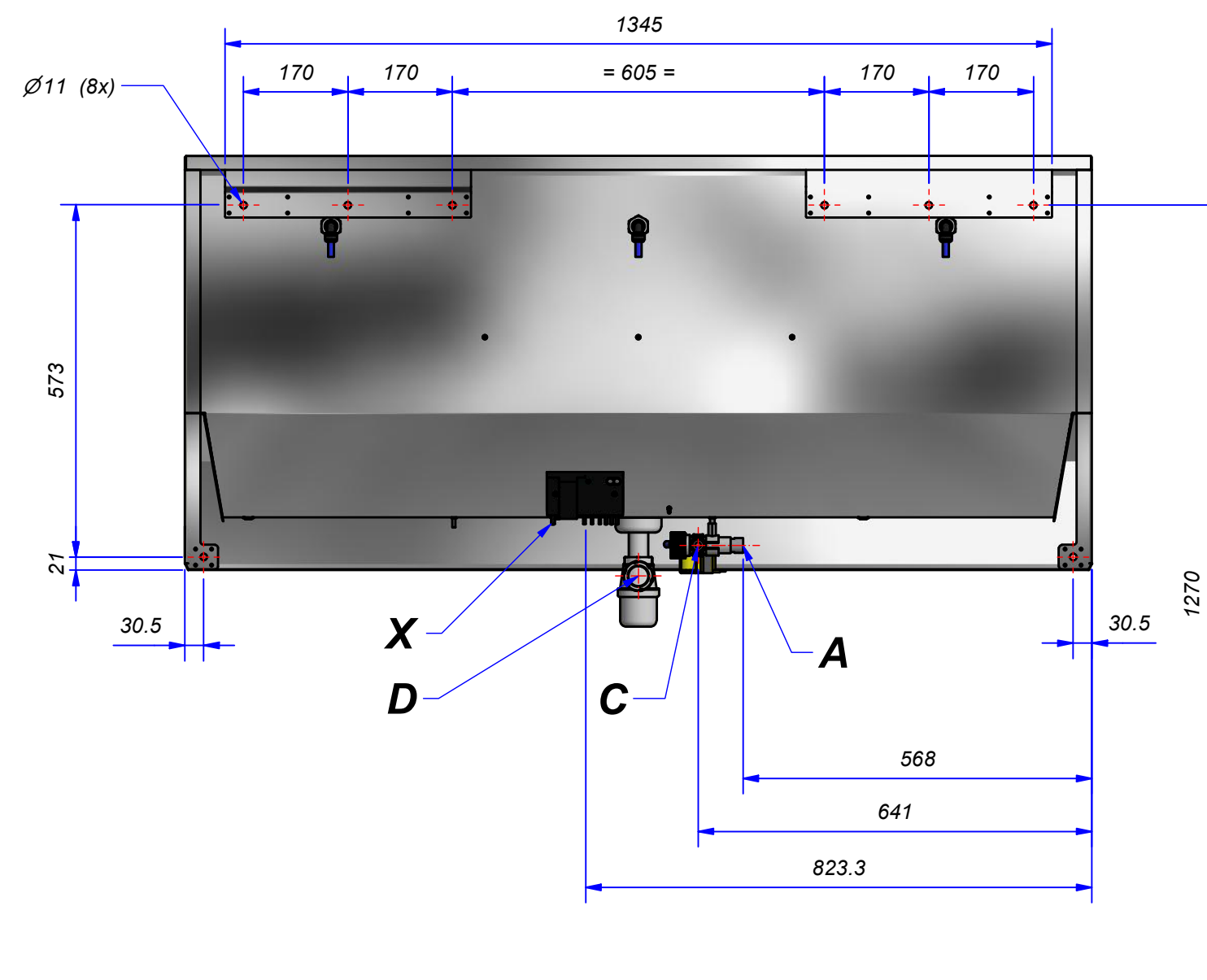
Back view E ( 1 : 10 )
